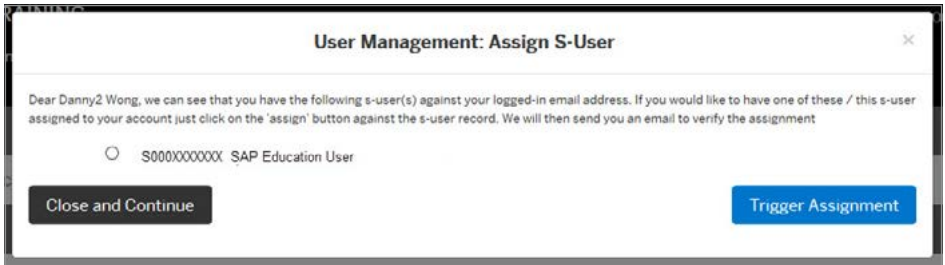
Figure 25: Assign S-User
