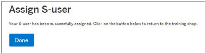
Figure 16: Successful Assignment
