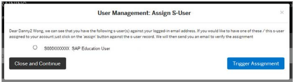
Figure 32: Assign S-User
