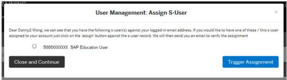
Figure 14: Assign S-User
